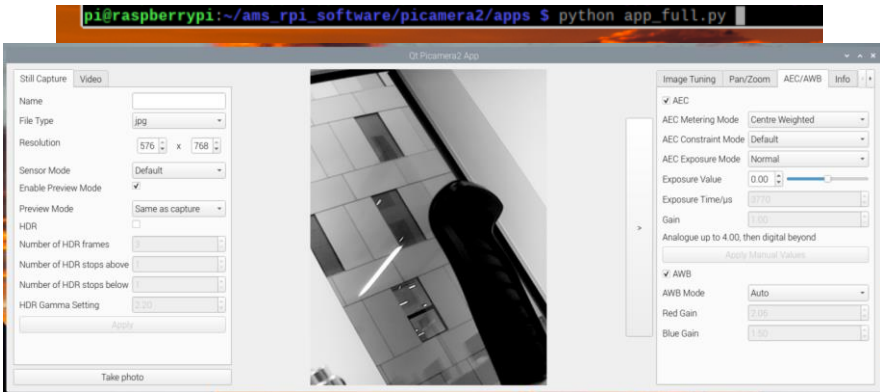
Figure 9: App_full.py
