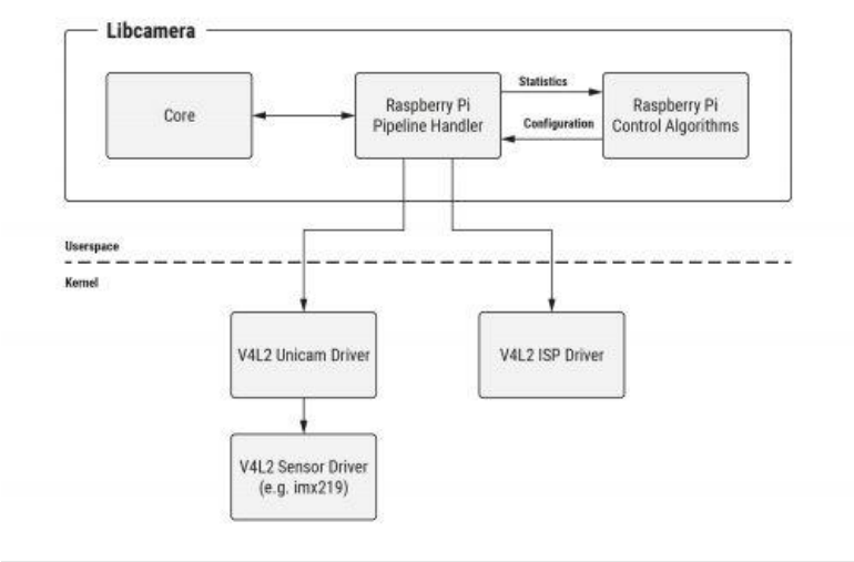
Figure 5: Camera framework architecture
